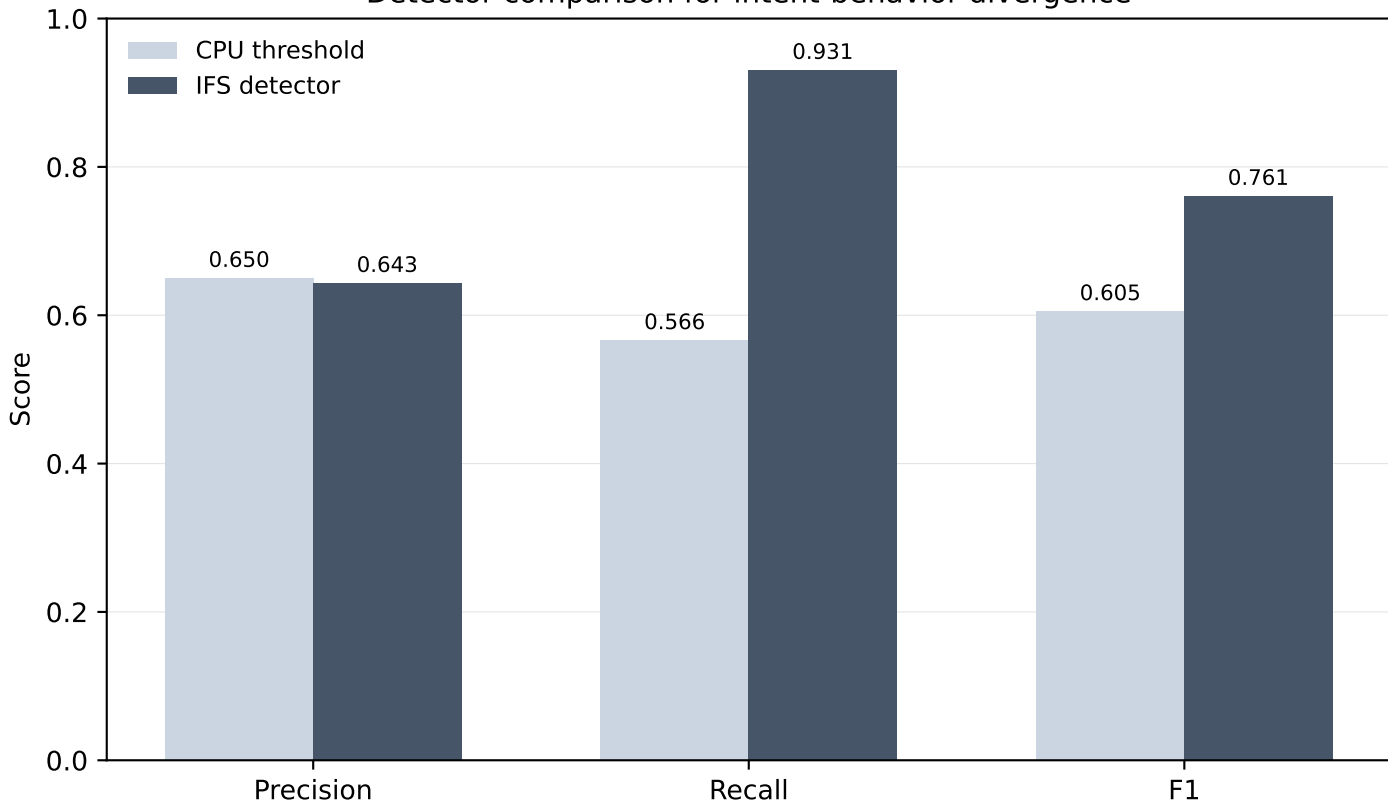
Detector comparison for intent-behavior divergence
