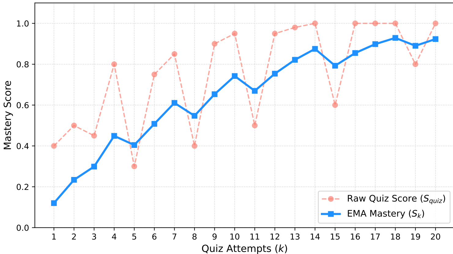
Stabilization of Concept Mastery via Exponential Moving Average (EMA)
