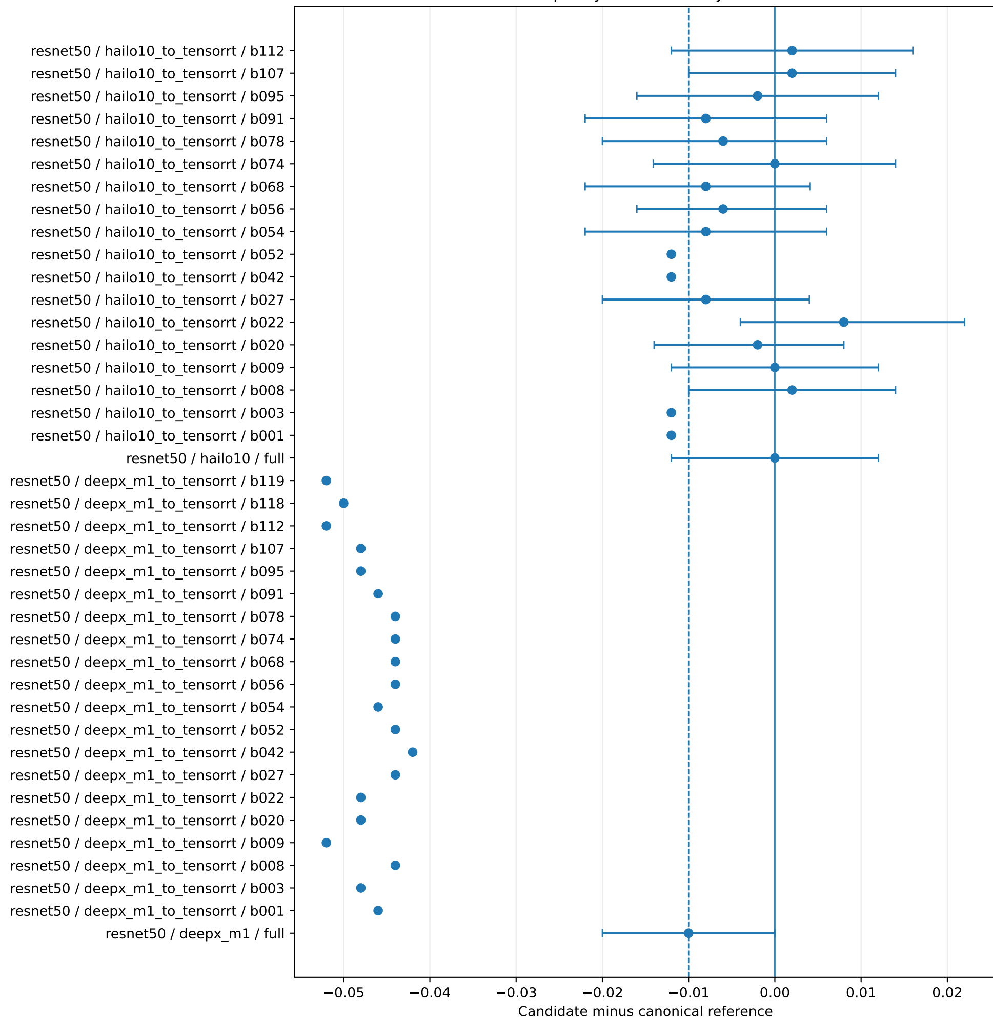
Task-quality non-inferiority results
