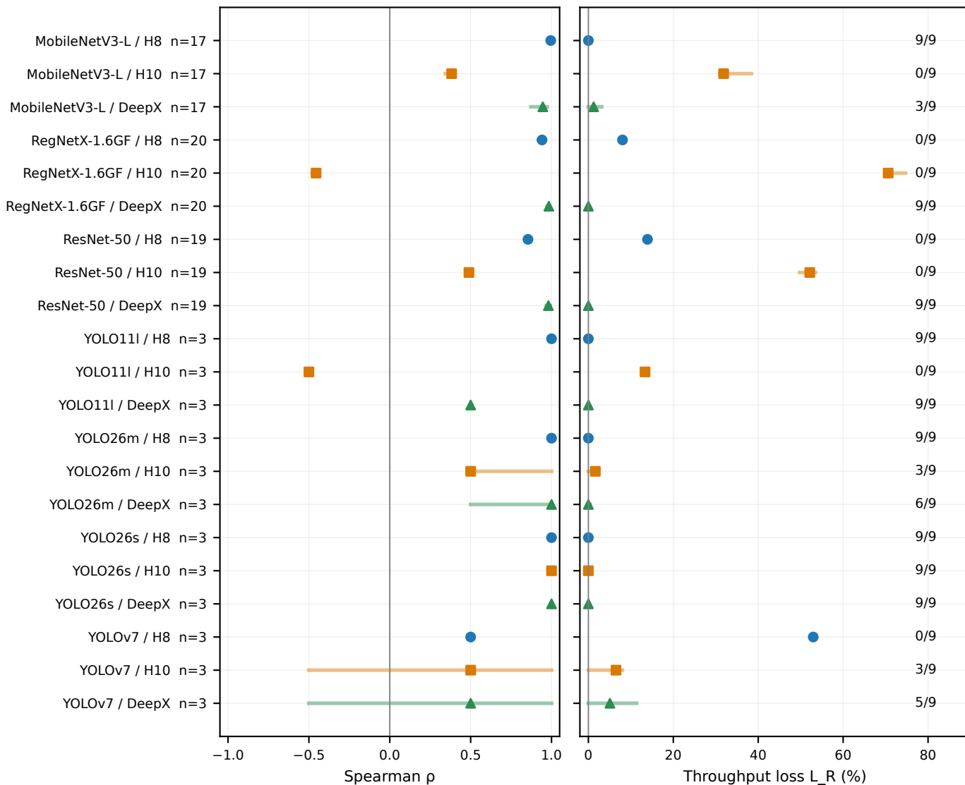
(a) Rank transfer
