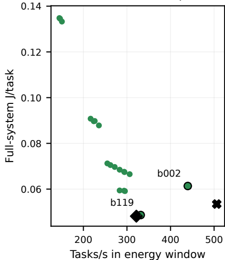
ResNet-50 / DeepX
