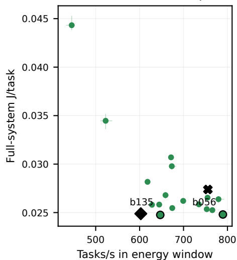
MobileNetV3-L / DeepX
