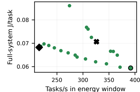
ResNet-50 / DeepX
