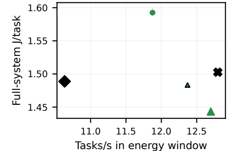
YOLOv7 / DeepX
