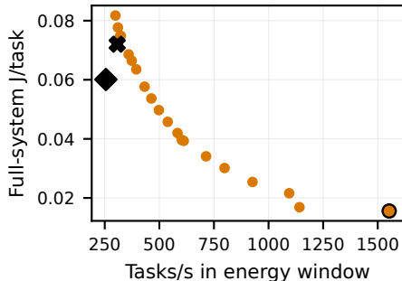
ResNet-50 / H10
