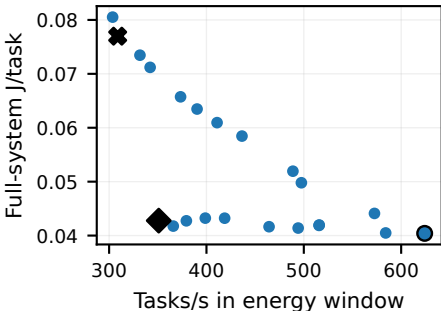
ResNet-50 / H8
