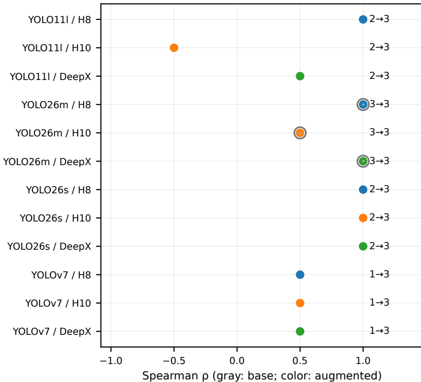
(a) Exact completed-task rank groups; n base→new
