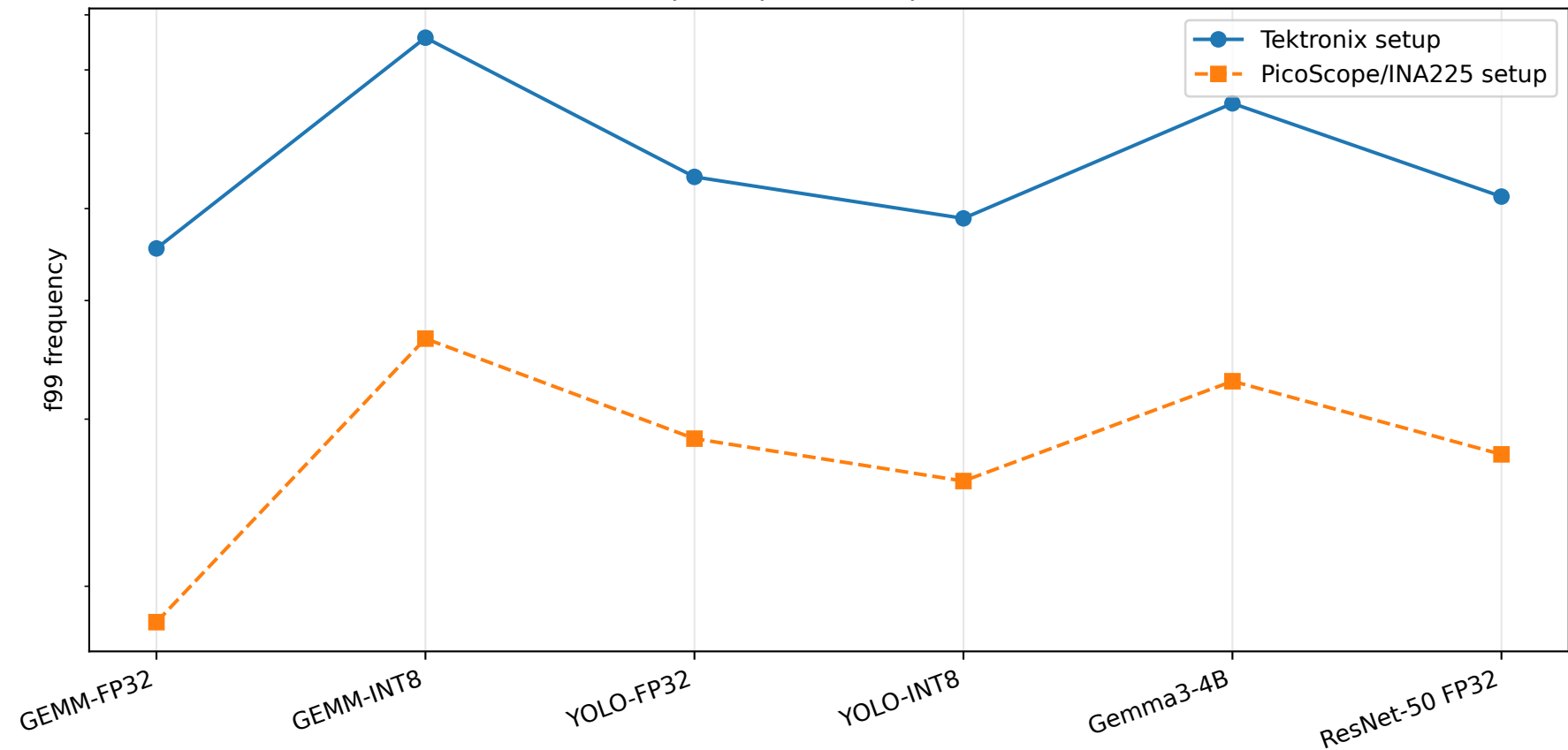
Setup comparison of power f99
