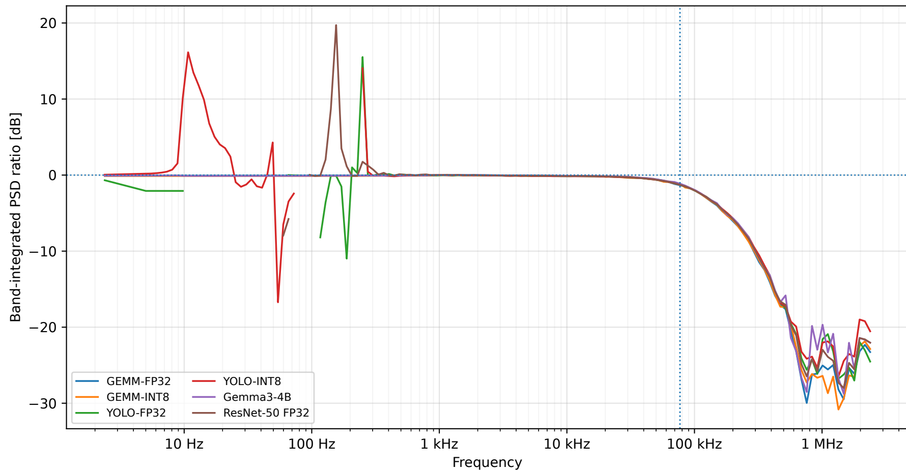
Observed Pico/Tek power PSD ratio
