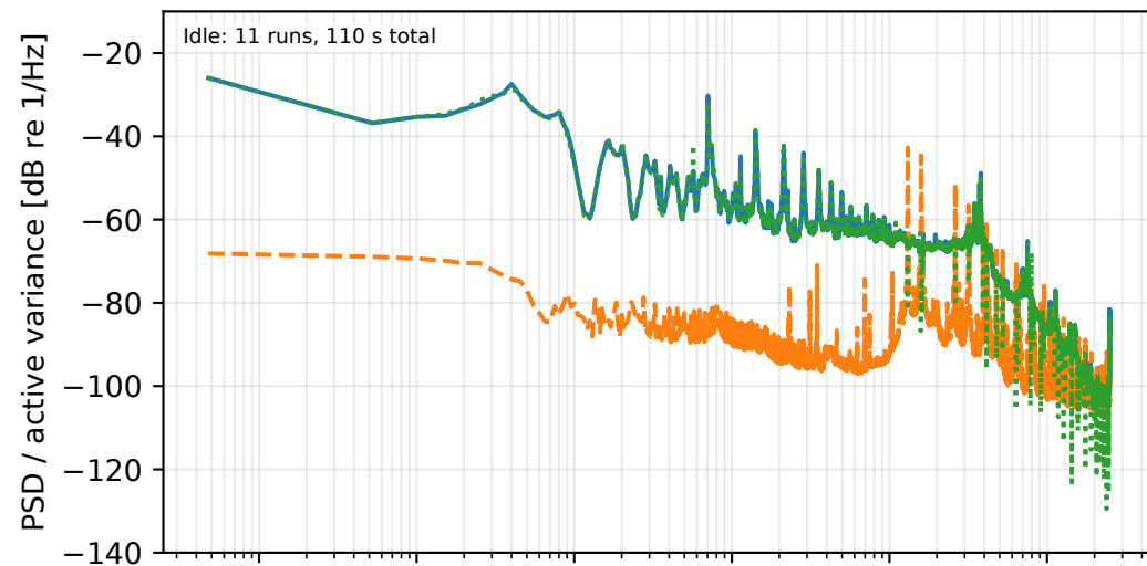
(c) YOLO-FP32
