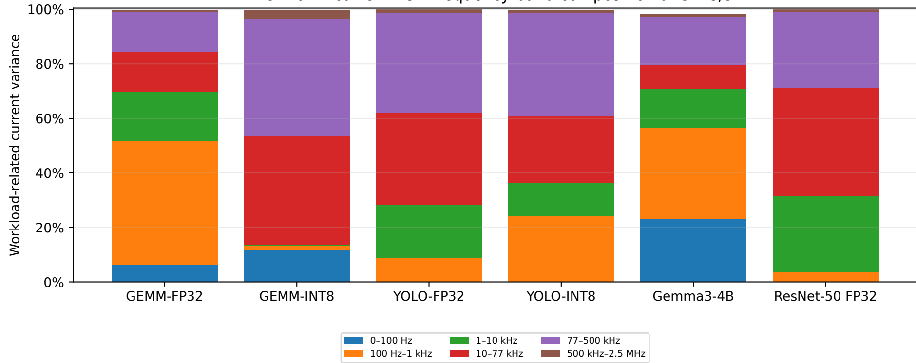
Tektronix current-PSD frequency-band composition at 5 MS/s
