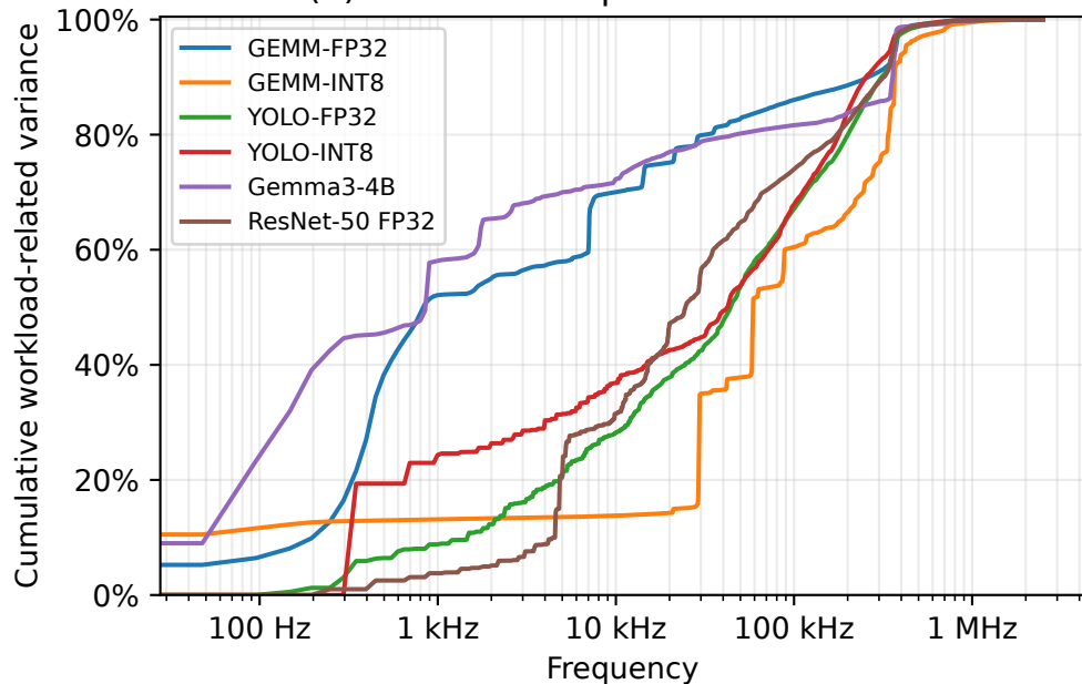
(b) Cumulative spectral distribution
