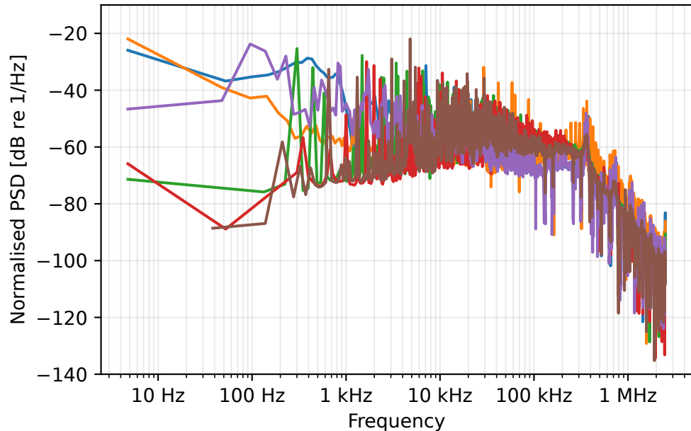
(a) Tektronix power PSD shape at 5 MS/s
