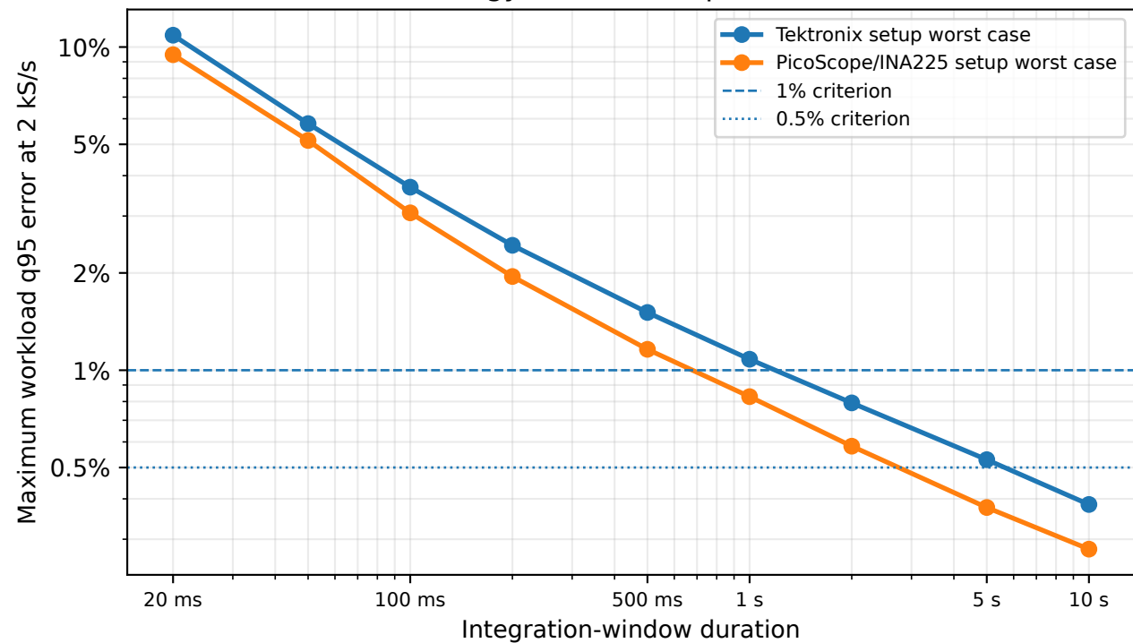
Conservative 2-kS/s energy-error envelope across available workloads
