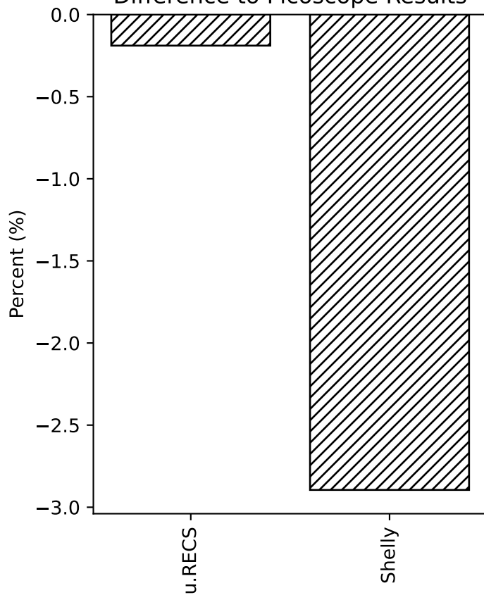
Difference to Picoscope Results
