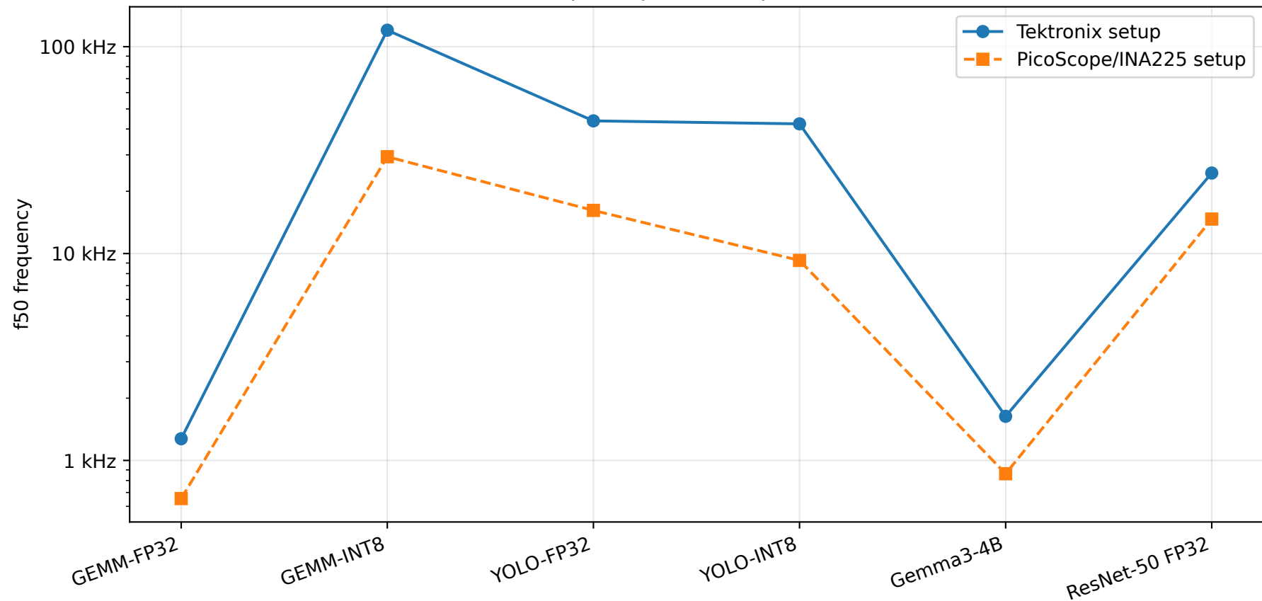
Setup comparison of power f50
