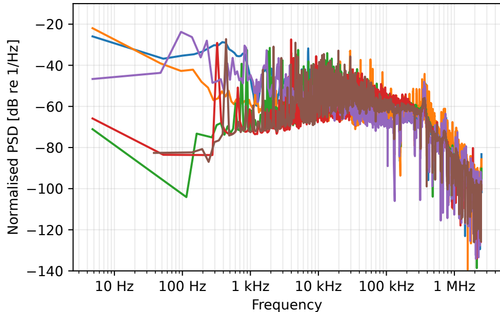
(a) Tektronix current PSD shape at 5 MS/s
