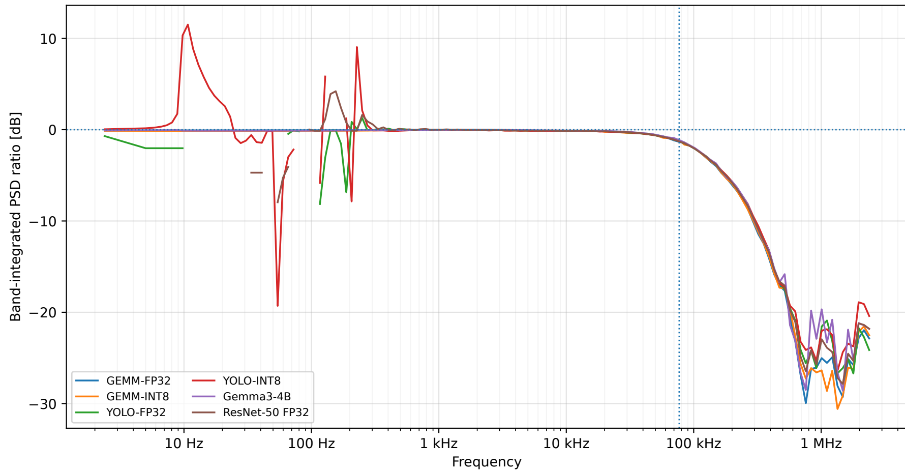
Observed Pico/Tek current PSD ratio
