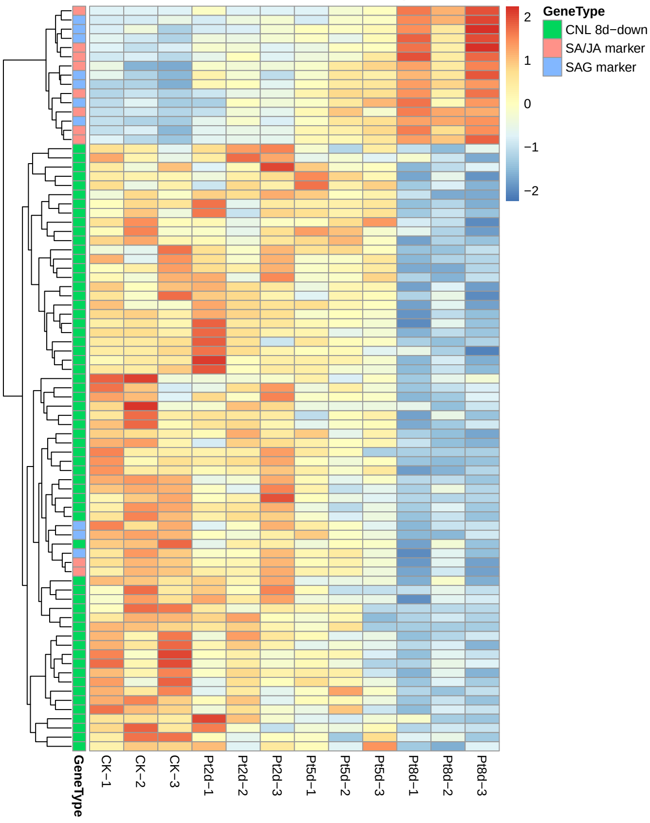
CNL 8d-down vs SA/JA & SAG markers (VST z-score)
