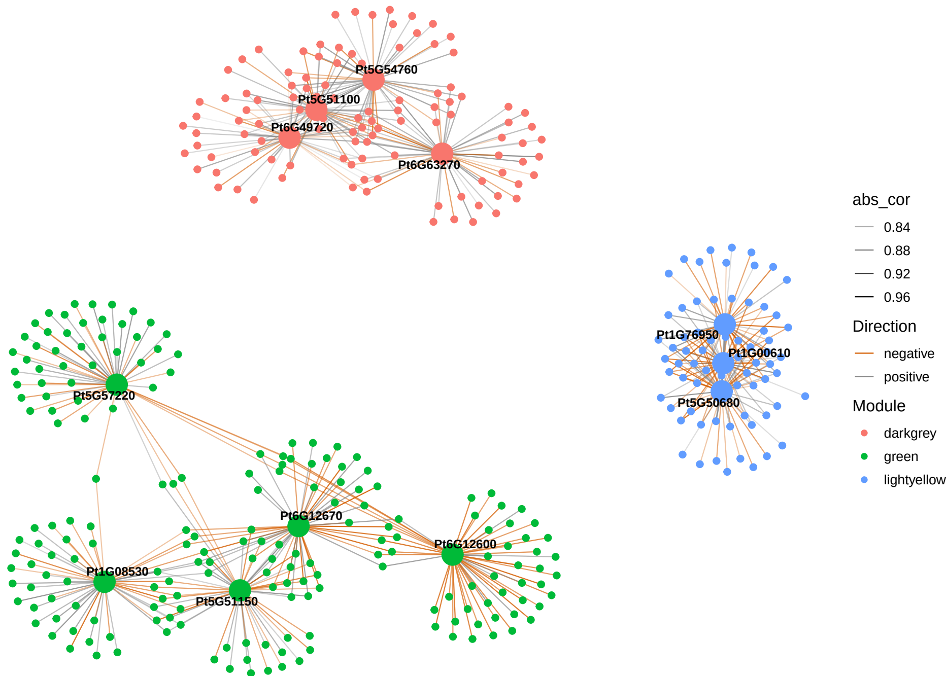
B. Top-12 hub NLR subnetwork 383 nodes, 602 edges; large nodes = top-hub NLRs
