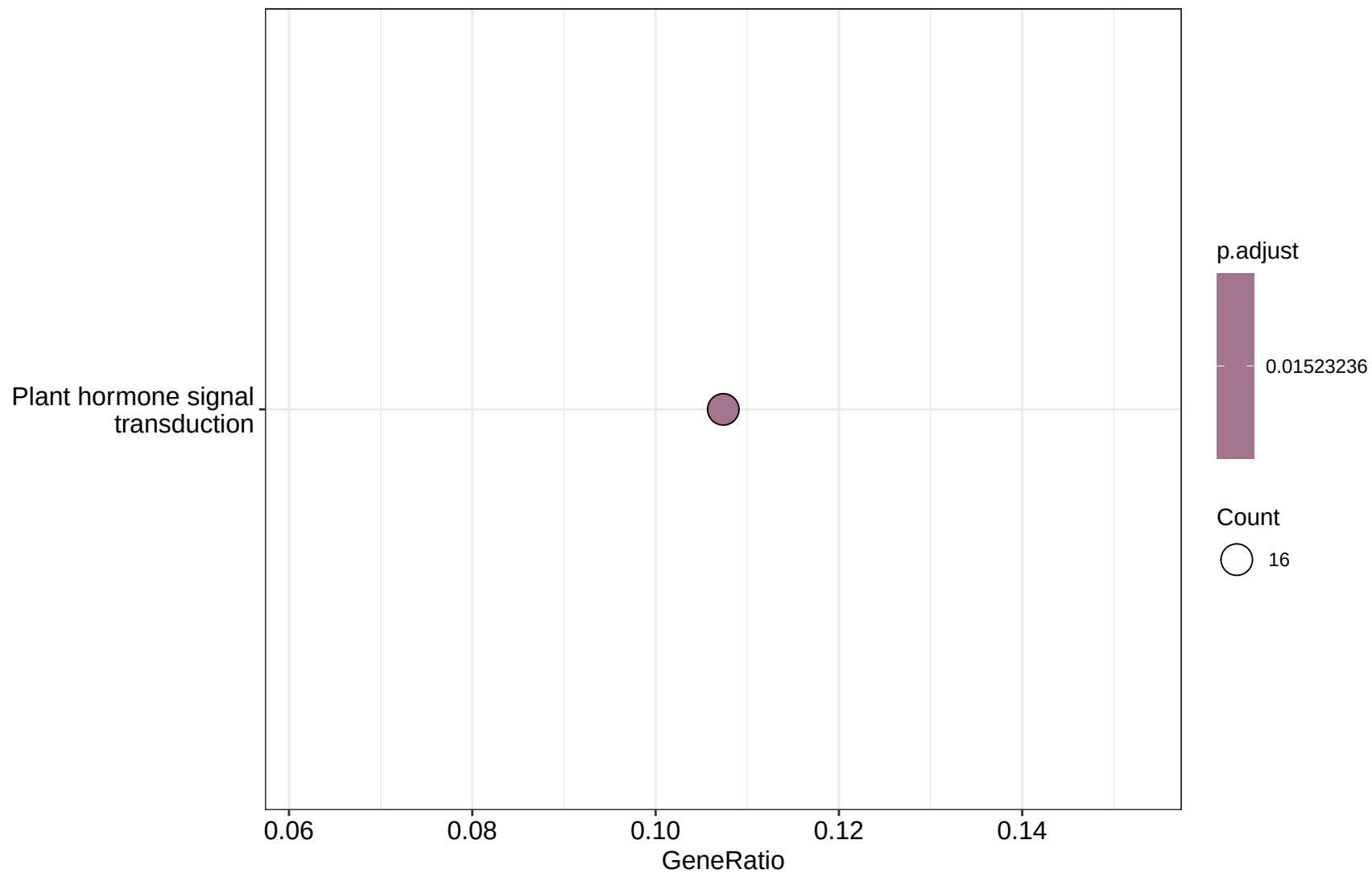
D-2. KEGG enrichment of NLR-network target genes
