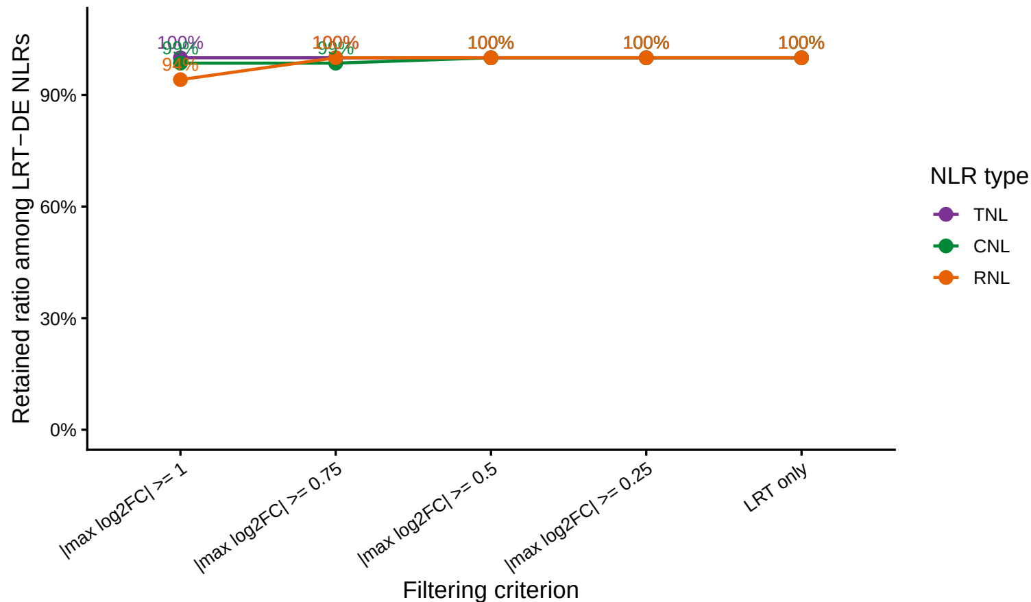
Proportion of LRT-DE NLRs retained under different log2FC thresholds
