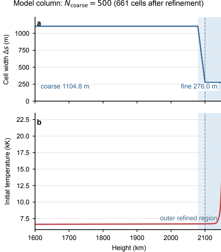
Figure 1: Release mesh and EOS-aware initial temperature for the coarse-equivalent N = 500 column. The mesh is reconstructed with the same static outer-refinement algorithm used by model_column .
