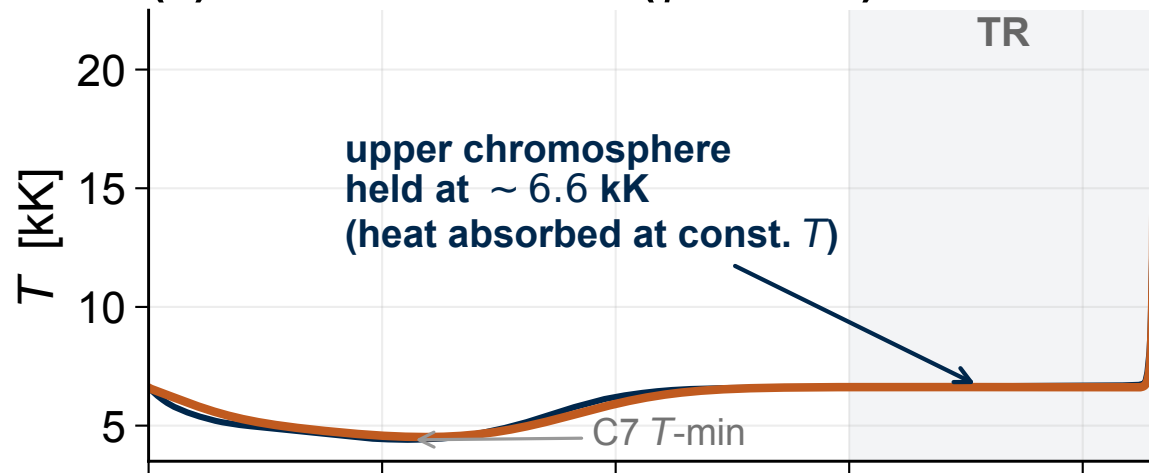
(a) Near-isothermal ( \gamma = 1.05 )
