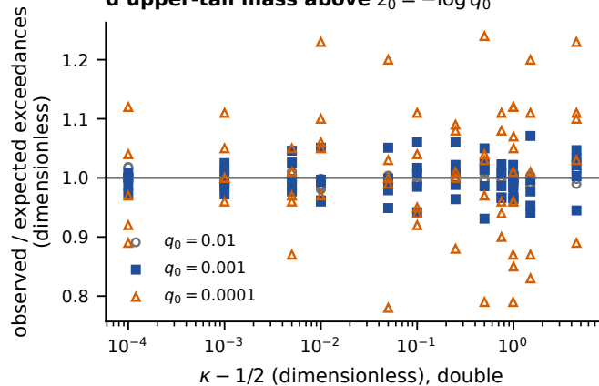
d upper-tail mass above z_0 = -\log q_0
