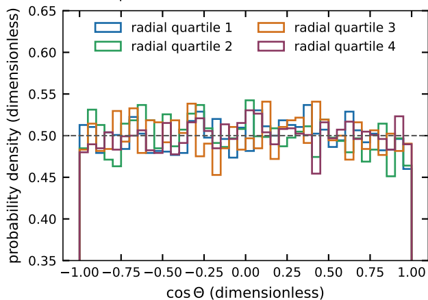
(c) independence of R and direction, \kappa = 2
