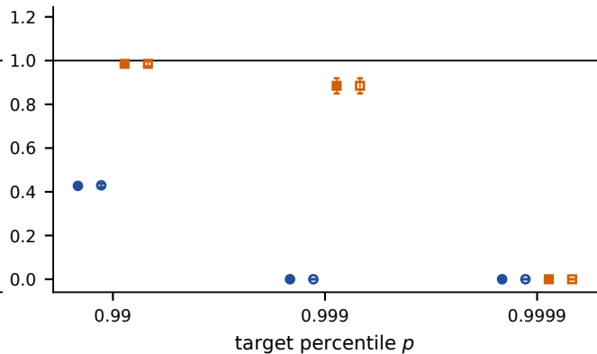
d float, \kappa = 0.55
