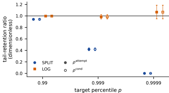
c double, \kappa = 0.51
