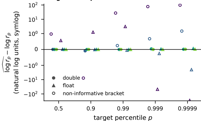
c log-radius quantile error
