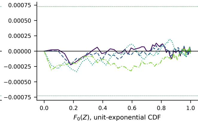
d upper-tail mass above z_0 = -\log q_0
