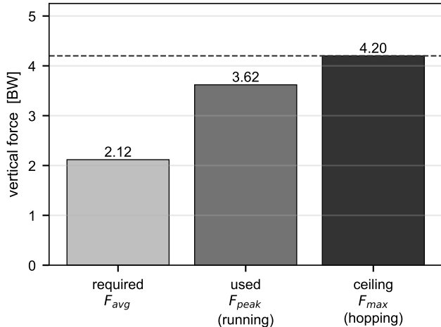
B force budget: peak used lies below the ceiling
