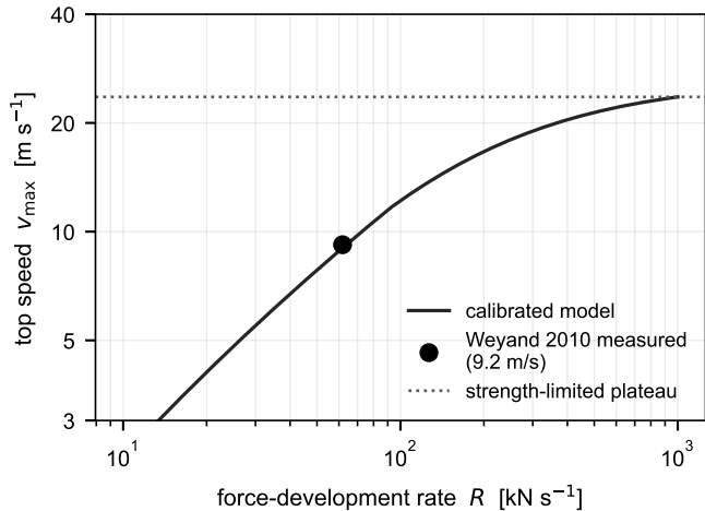
A calibrated v_{\max}(R) and its calibration point
