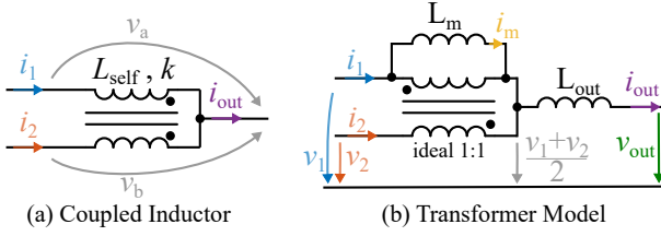
Fig. 3: The coupled inductor can be described with a self-inductance L_{self} and coupling factor k or by using an equivalent circuit consisting of an ideal 1:1 transformer with magnetizing inductance L_m and common output inductance L_{out} .
