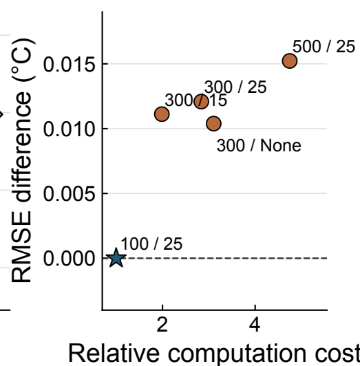
f Model cost trade-off
