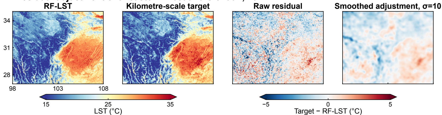
f Residual adjustment over eastern Tibet and Sichuan, 2024
