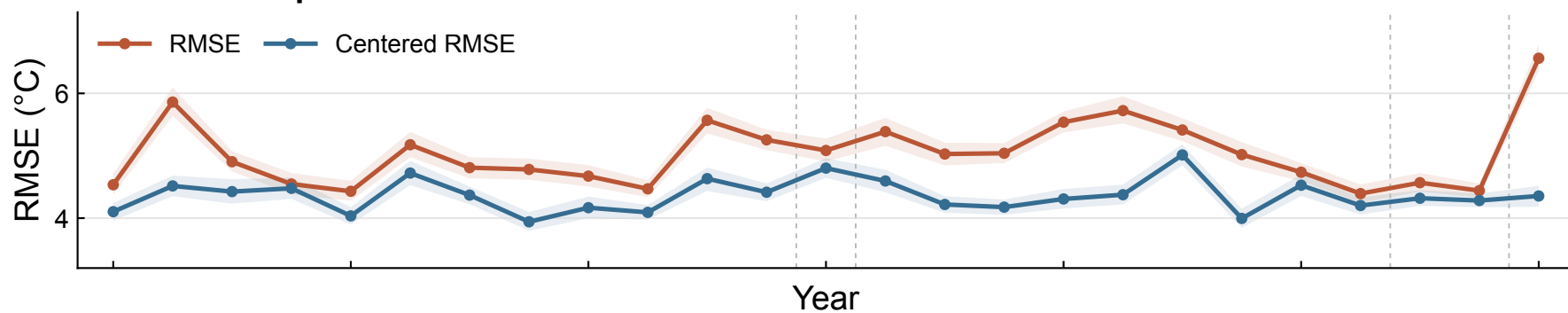
b Annual temperature differences
