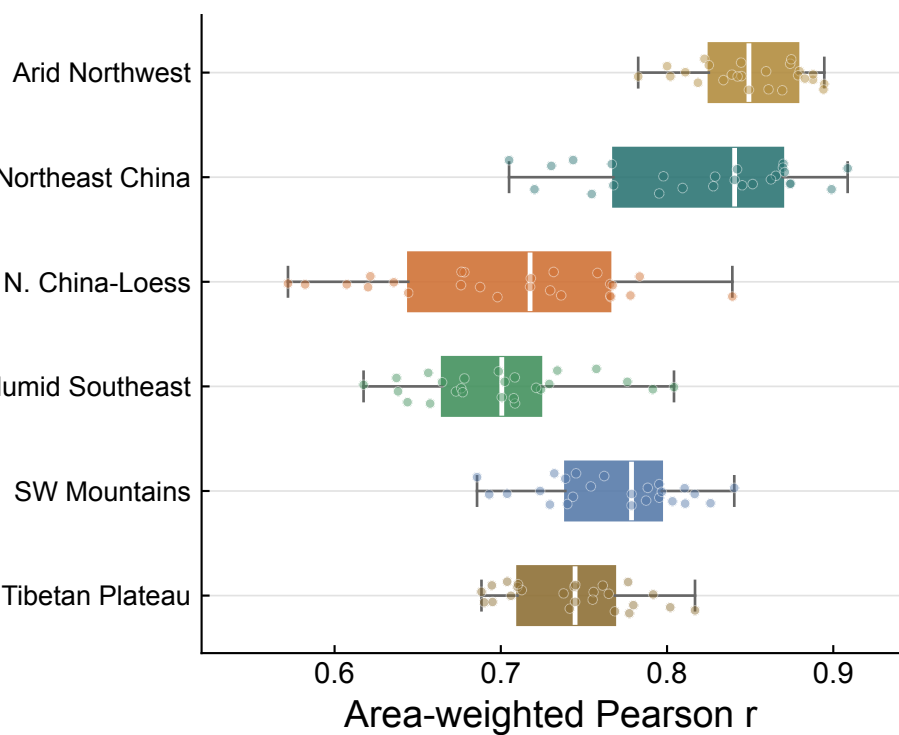
c Macroregional spatial agreement
