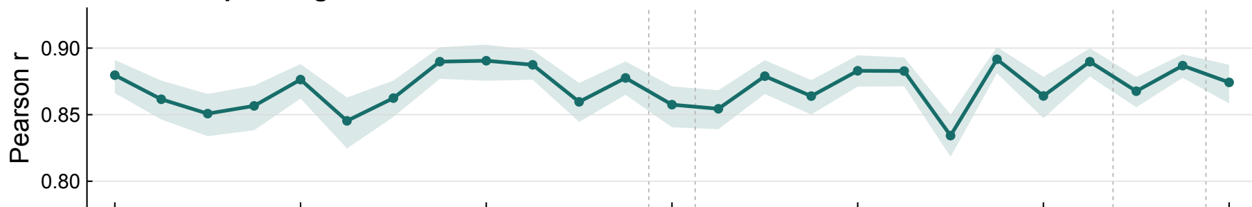
a Annual spatial agreement with Landsat ST
