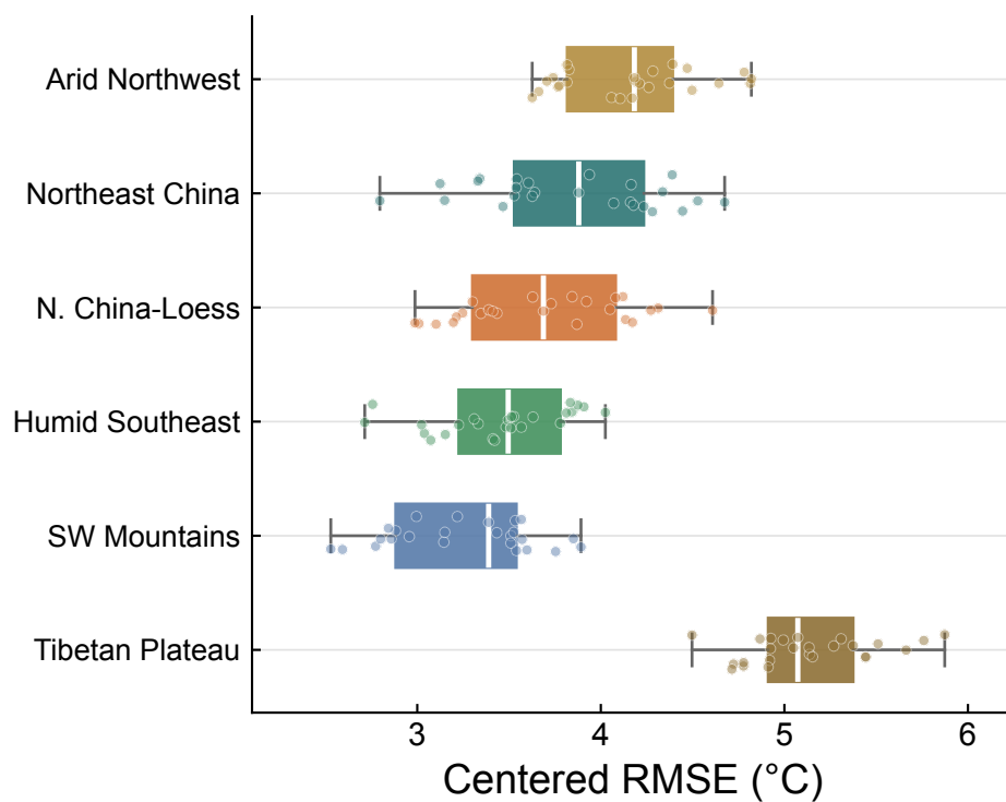
d Macroregional centered differences
