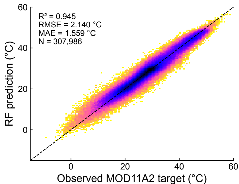
a Random 70/30 baseline
