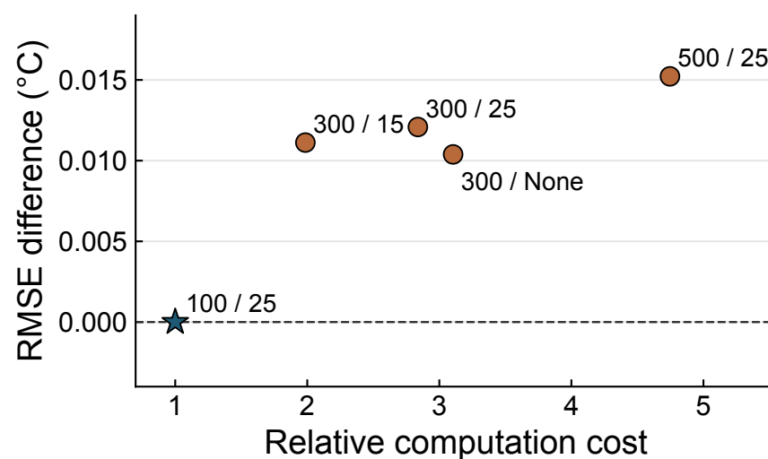
f Model cost trade-off
