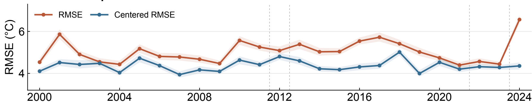
b Annual temperature differences
