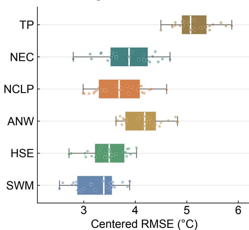
d Macroregional centered differences
