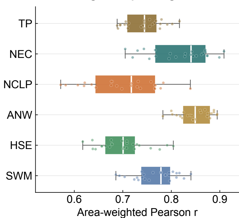
c Macroregional spatial agreement
