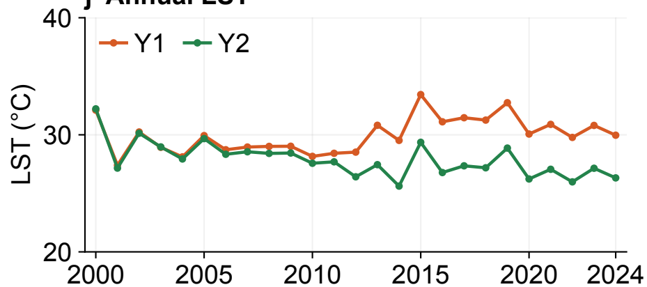
j Annual LST
