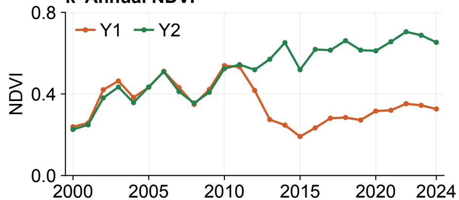
k Annual NDVI
