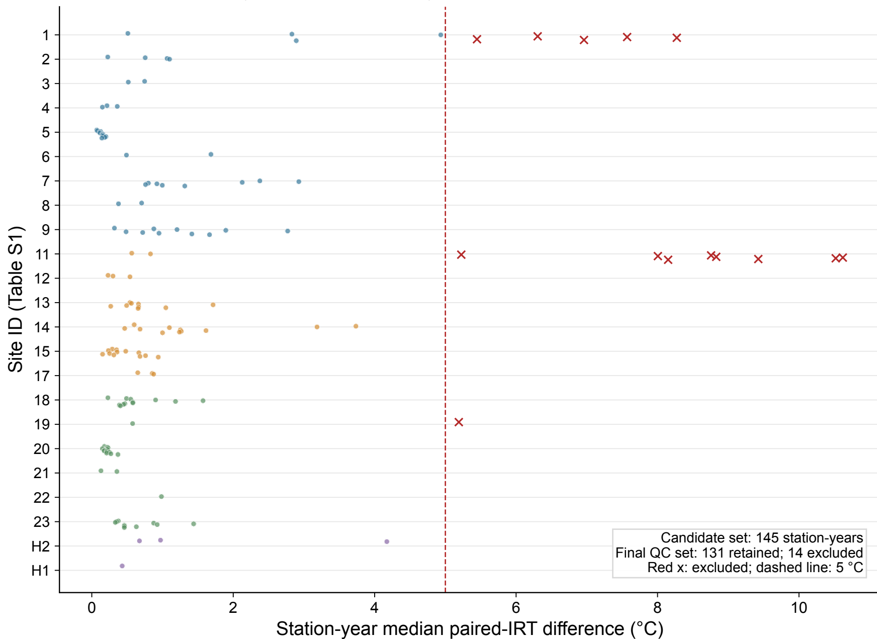
Paired-IRT consistency of candidate station-years
