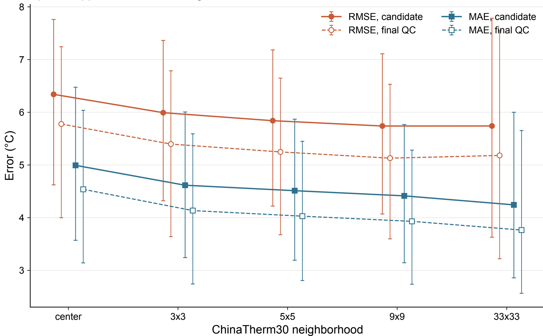
Spatial support before and after ground-reference QC
