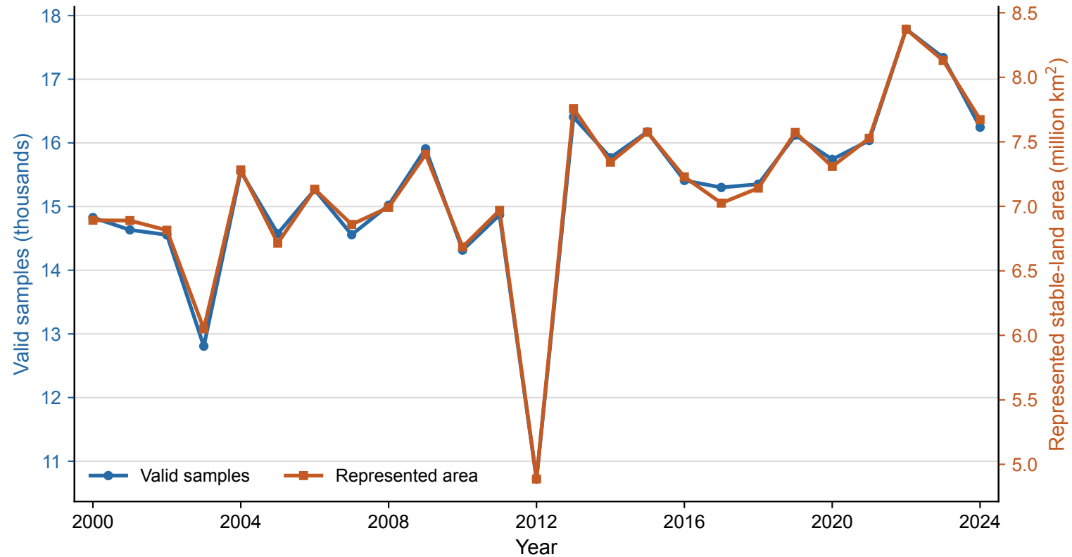
Annual support of the nationwide Landsat validation
