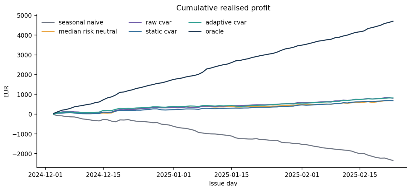
Figure 2. Cumulative simulated profit over the evaluation block; profit is unchanged by the reporting correction. Source: corrected v1.0.1 baseline, retained in v1.0.2.
