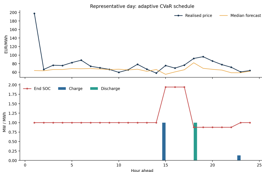
Figure 1. Representative adaptive-CVaR schedule, showing power and SOC feasibility and restoration of terminal SOC. Source: corrected v1.0.1 baseline, retained in v1.0.2.
