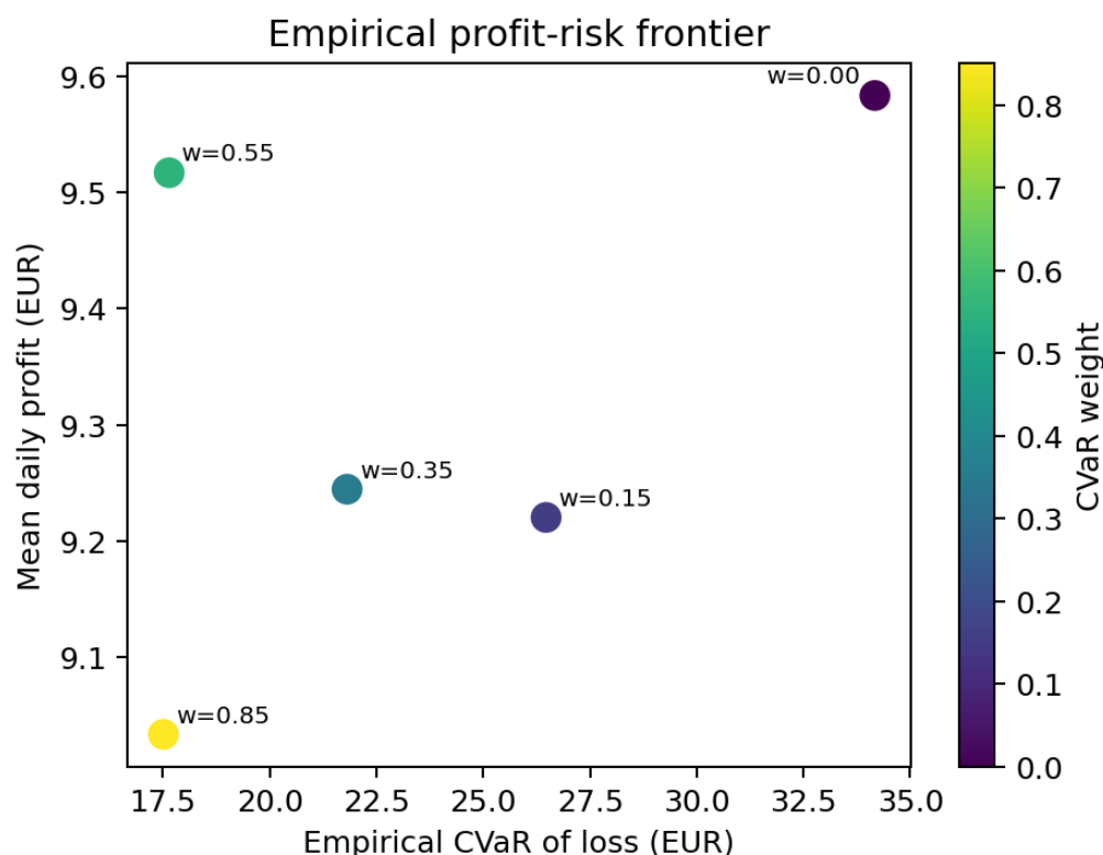
Figure 5. Mean simulated profit versus fixed-mass empirical CVaR loss, using a separate frontier scenario sample. Source: corrected v1.0.1 baseline table; labels redrawn for v1.0.2.
