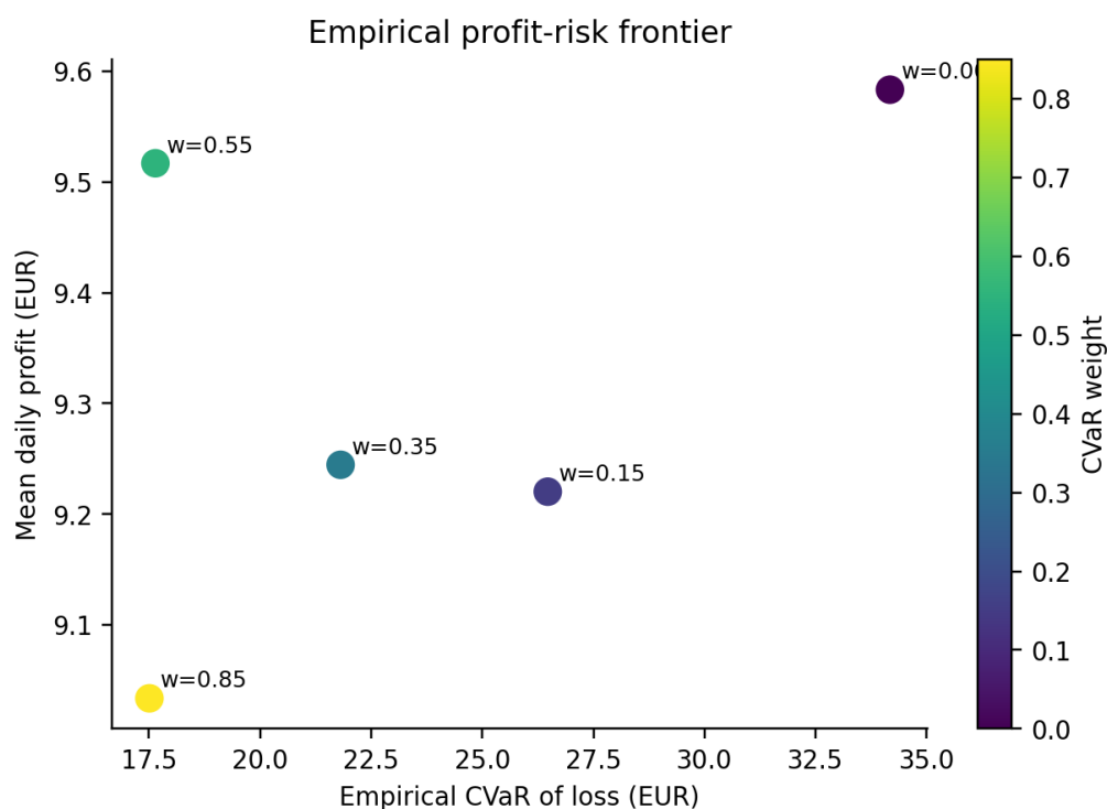
Figure 5. Mean simulated profit versus fixed-mass empirical CVaR loss, using a separate frontier scenario sample. Source: regenerated v1.0.1 baseline.
