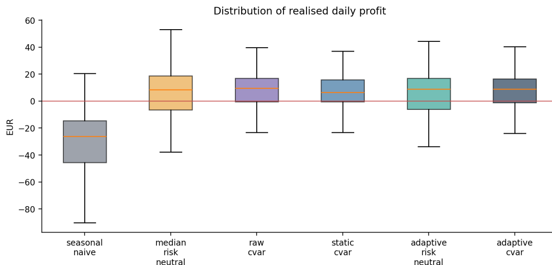
Figure 3. Simulated daily profit distributions for feasible benchmark strategies. Source: regenerated v1.0.1 baseline.
