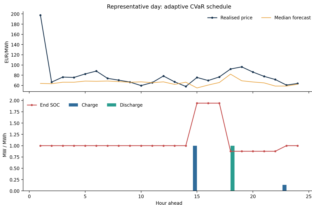
Figure 1. Representative adaptive-CVaR schedule, showing power and SOC feasibility and restoration of terminal SOC. Source: regenerated v1.0.1 baseline.
