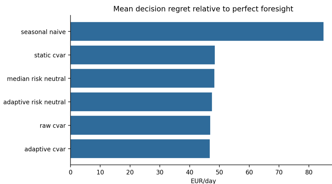
Figure 4. Mean daily regret relative to the perfect-foresight oracle; lower is better. Source: regenerated v1.0.1 baseline.
