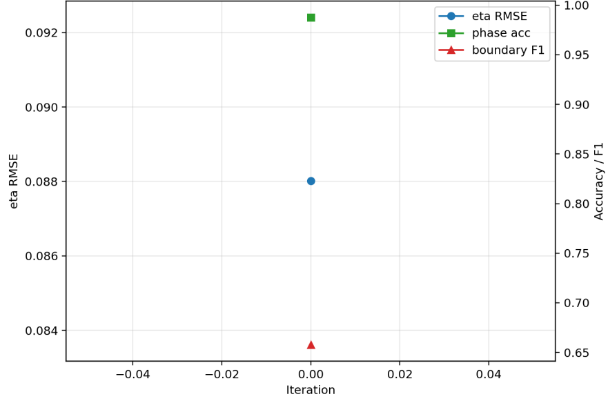
Figure 3: Learning-curve summary.
