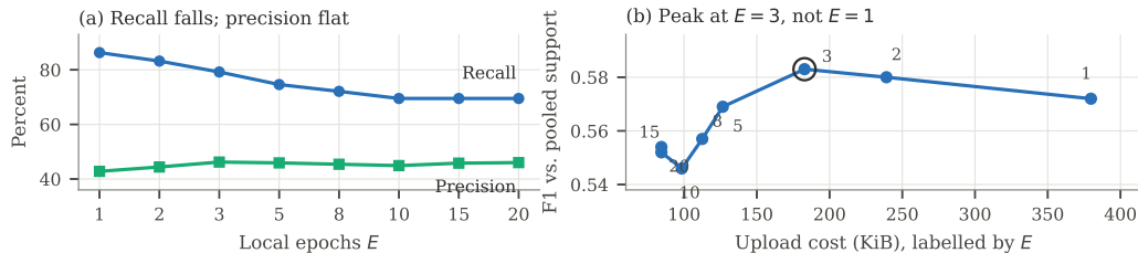
Figure 1: Recall declines monotonically in E while precision is flat (a), so agreement with the centralized fit peaks in the interior at E = 3 rather than at E = 1 (b). In this single run, reducing communication from E = 1 to E = 3 did not reduce observed F1.
