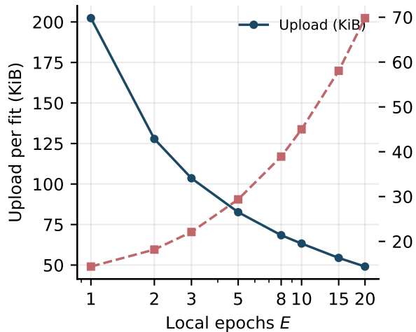
Independent
