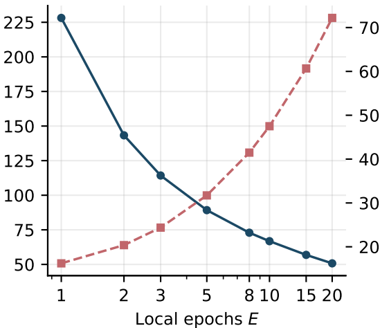
Correlated
