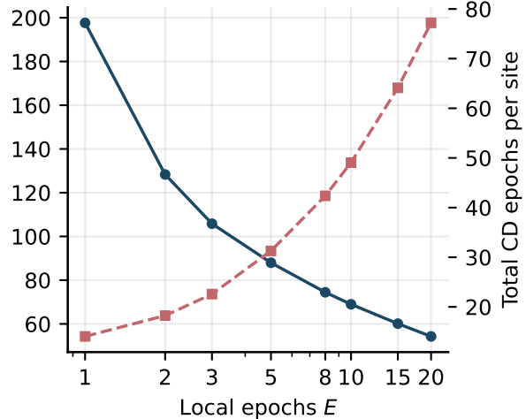
Heterogeneous
