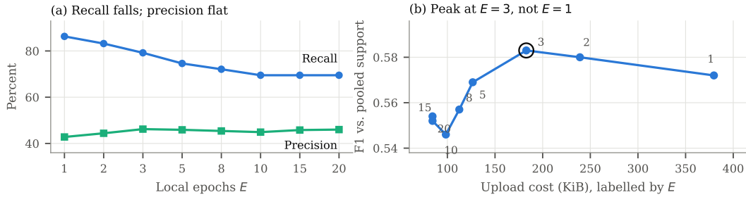
Figure 1: Recall declines monotonically in E while precision is flat (a), so agreement with the centralized fit peaks in the interior at E = 3 rather than at E = 1 (b). In this single run, reducing communication from E = 1 to E = 3 did not reduce observed F1.
