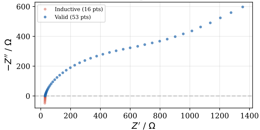
(a) Raw Data (69 pts, 7 MHz \rightarrow 1 Hz)
