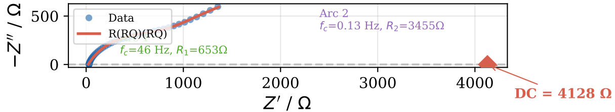
(b) R(RQ)(RQ) Fit ( \chi^2/N=23.0 )
