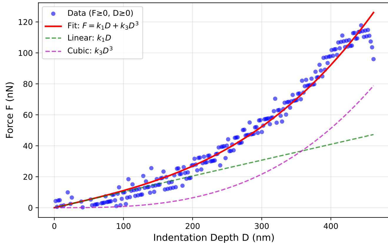
linker2 - Best Fit ( R^2 = 0.979 ) k80-linker2-paa-50nm-500nm-10uN - NanoScope Analys...
