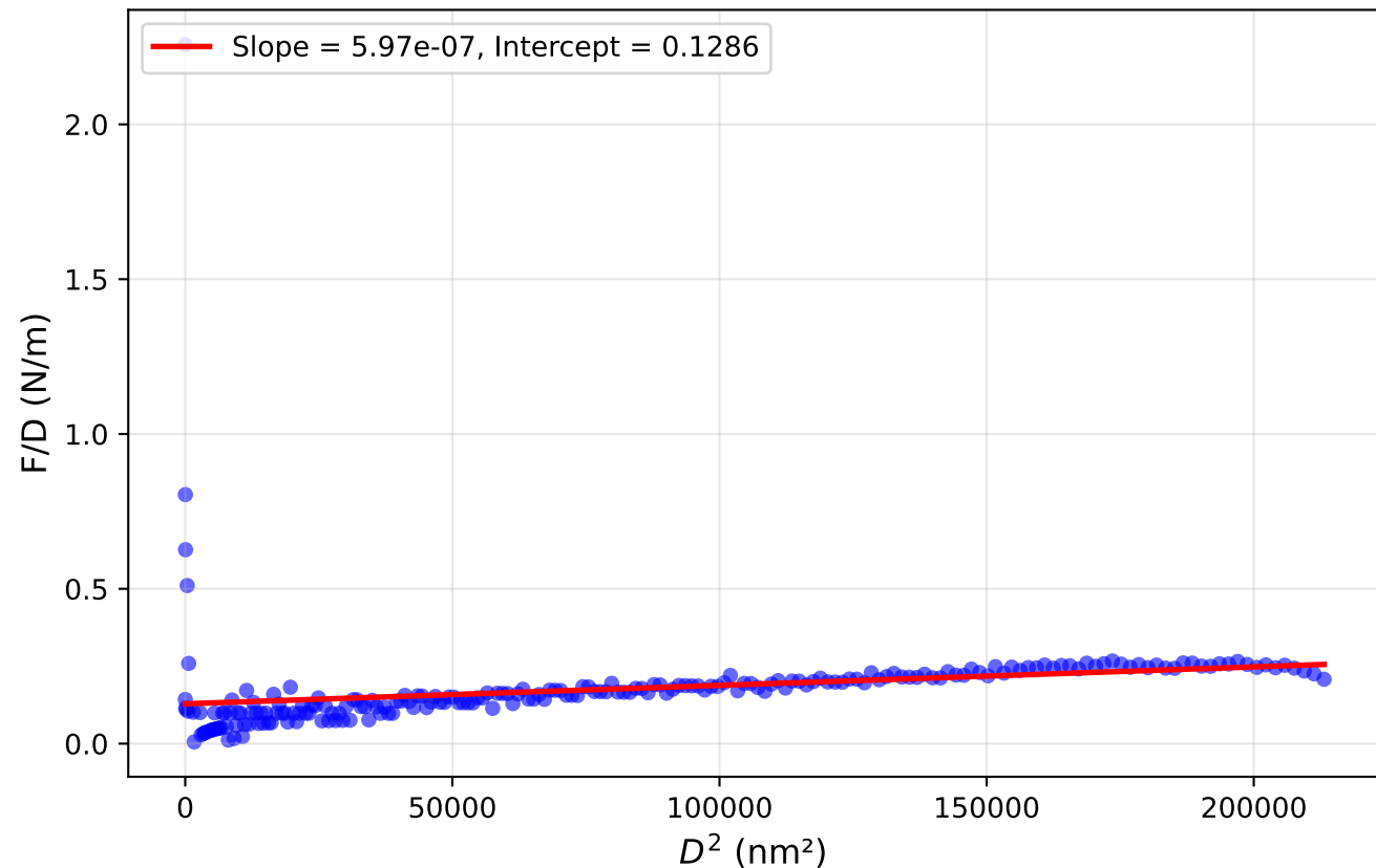
linker2 - Linearized: F/D = k_1 + k_3 D^2
