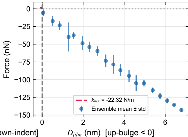
Negative region ( F < 0 ): k_{total} = k_{film} + k_{capillary}
