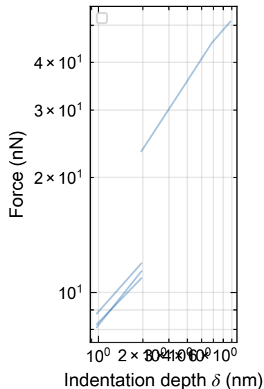
Force vs Indentation (log-log)
