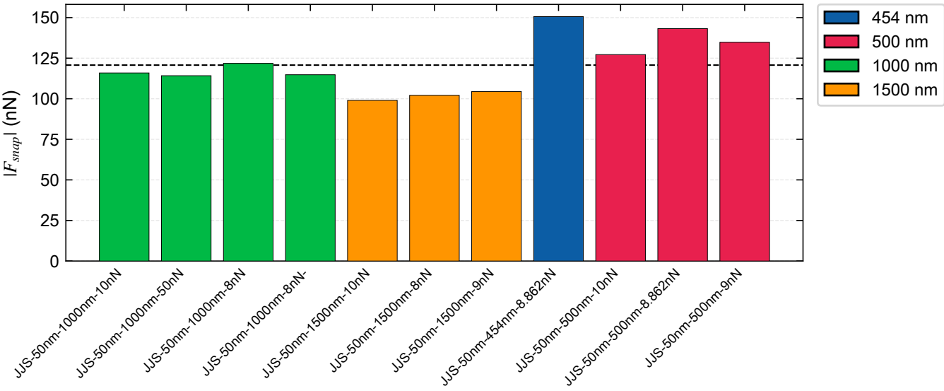
Snap-in Force Magnitude (All 11 Curves)
