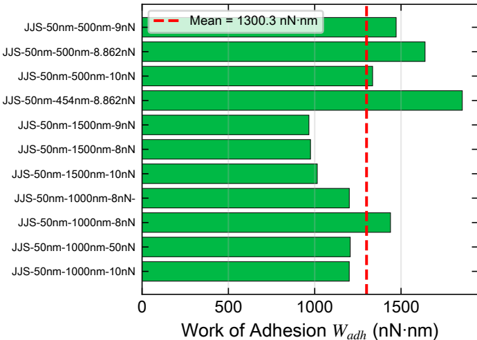
Work of Adhesion (per curve)
